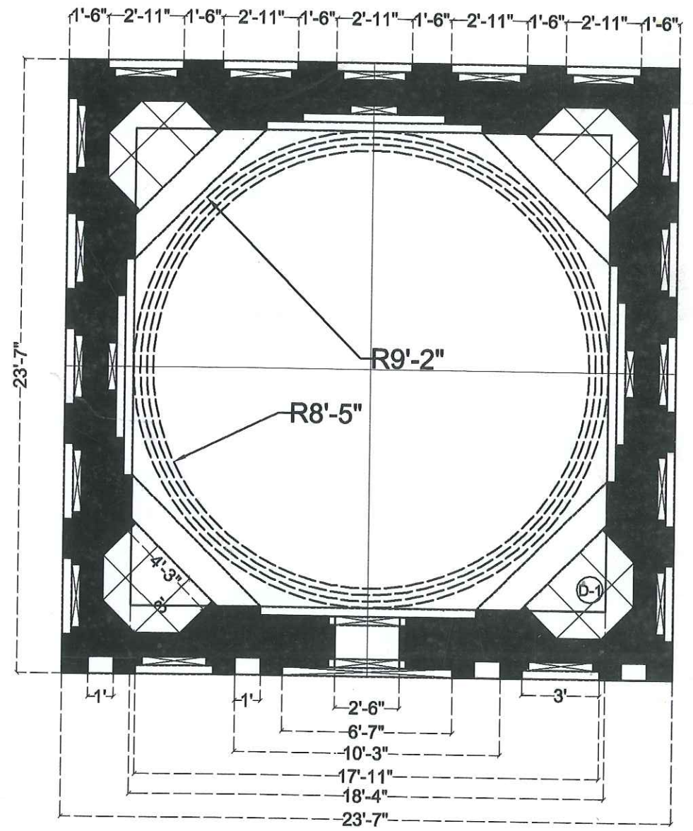
PLAN OF TOMB 01
