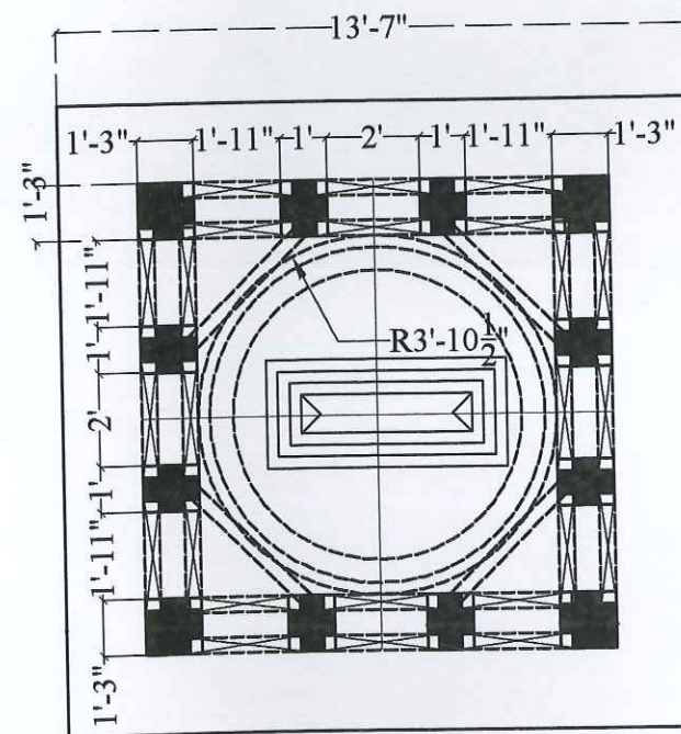
PLAN OF TOMB 05
