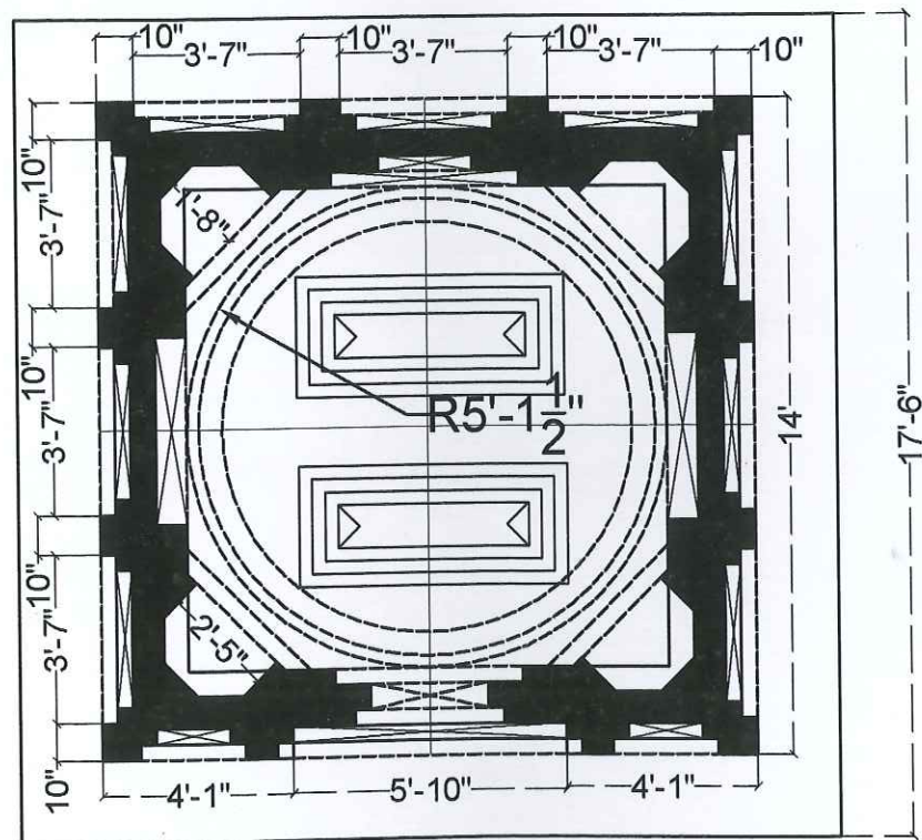
PLAN OF TOMB 07
