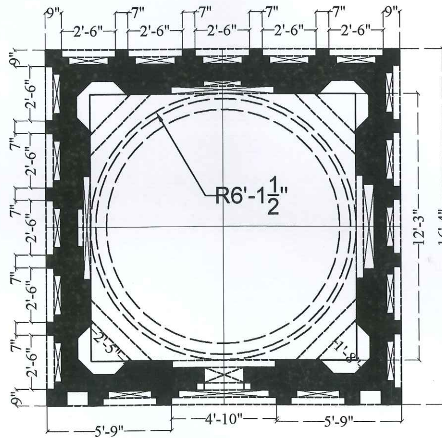
PLAN OF TOMB 04
