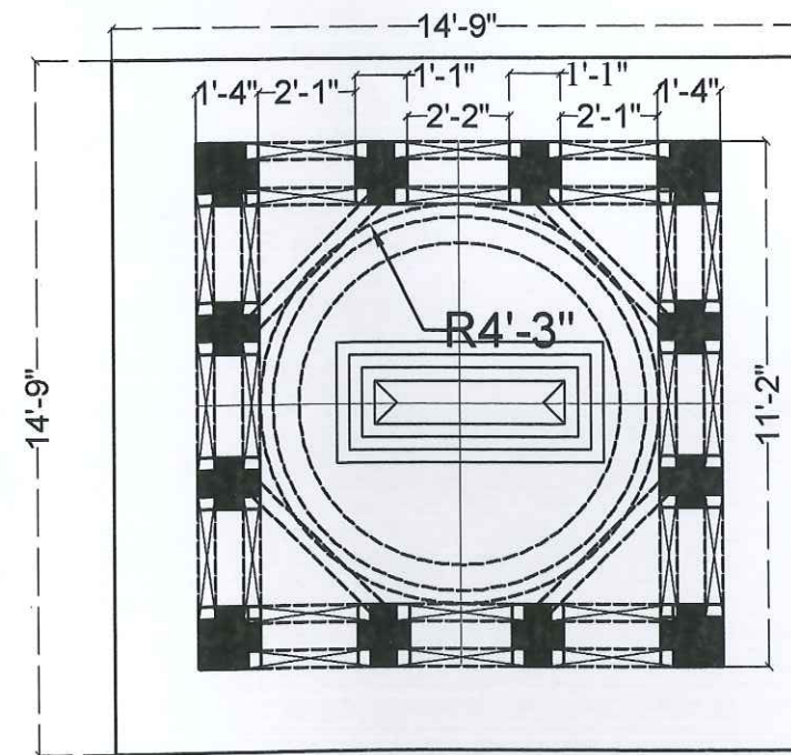
PLAN OF TOMB 06
