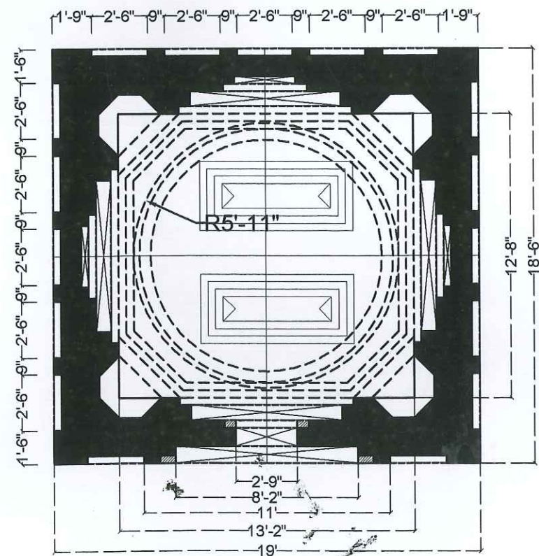
PLAN OF TOMB 10
