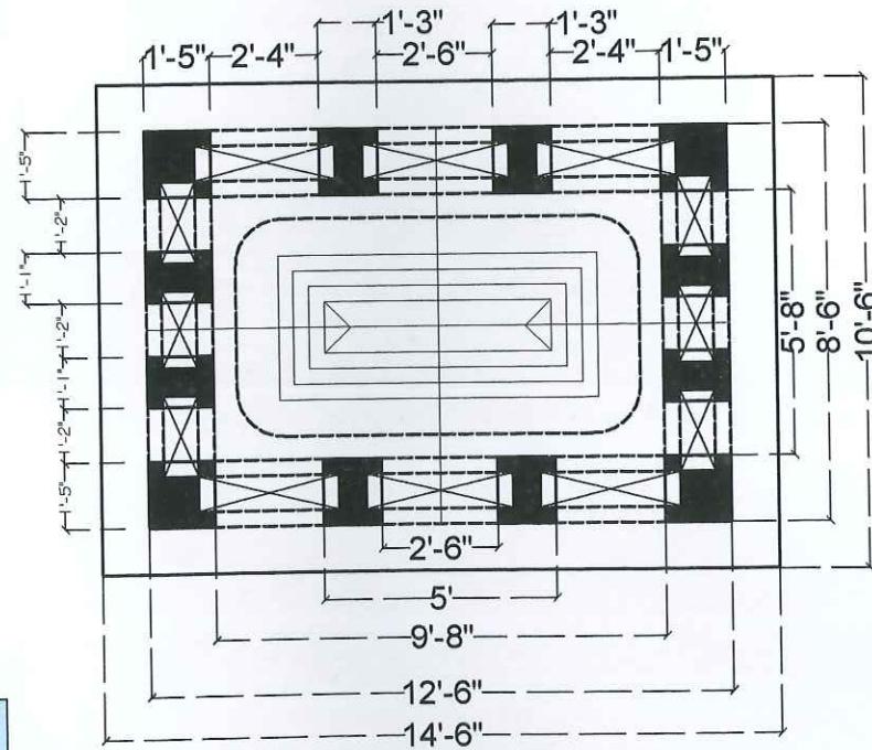
PLAN OF TOMB 09
