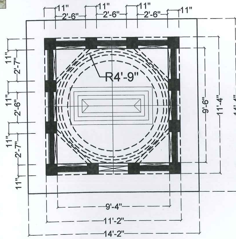
PLAN OF TOMB 11
