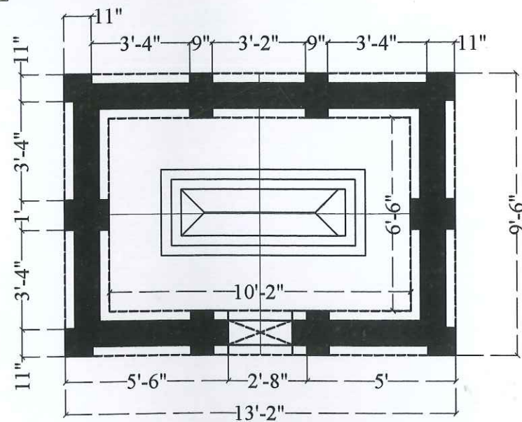
PLAN OF TOMB 03
